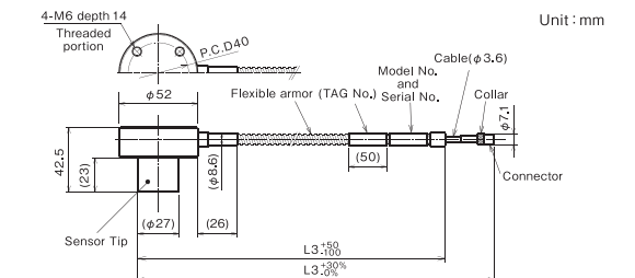
■ FL-143F28A (With armor (Without fluoro resin coating))
