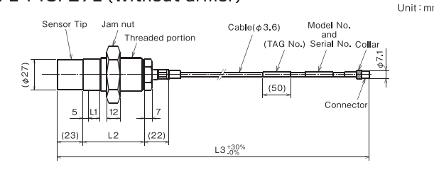
■ FL-143F27L (Without armor)
