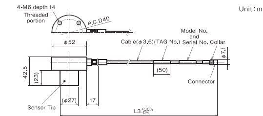
■ FL-143F28L (Without armor)
