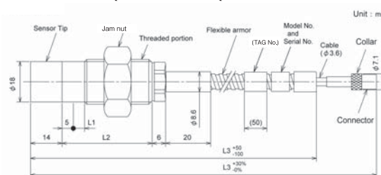
■ FL-602F18A (With armor (Without fluoro resin coating))
