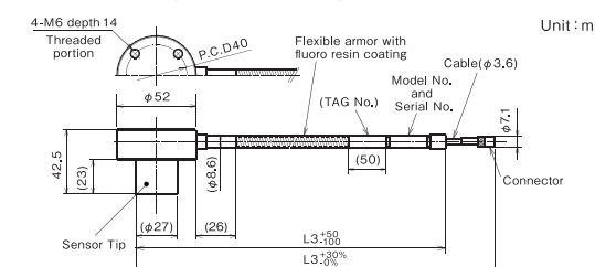
■ FL-143F28T (With armor (With fluoro resin coating))
