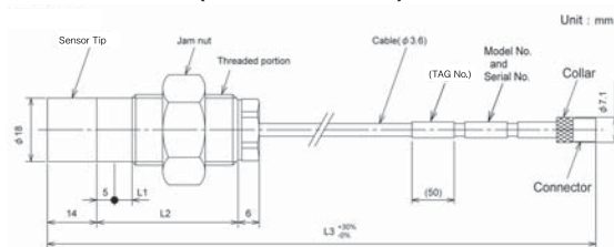
■ FL-602F18T (With armor (With fluoro resin coating))
