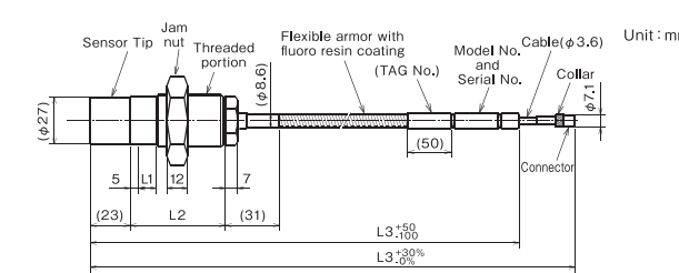
■ FL-143F27T (With armor (With fluoro resin coating))
