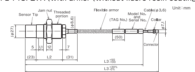
■ FL-143F27A (With armor (Without fluoro resin coating))
